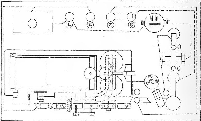
Military Morse recorder.
